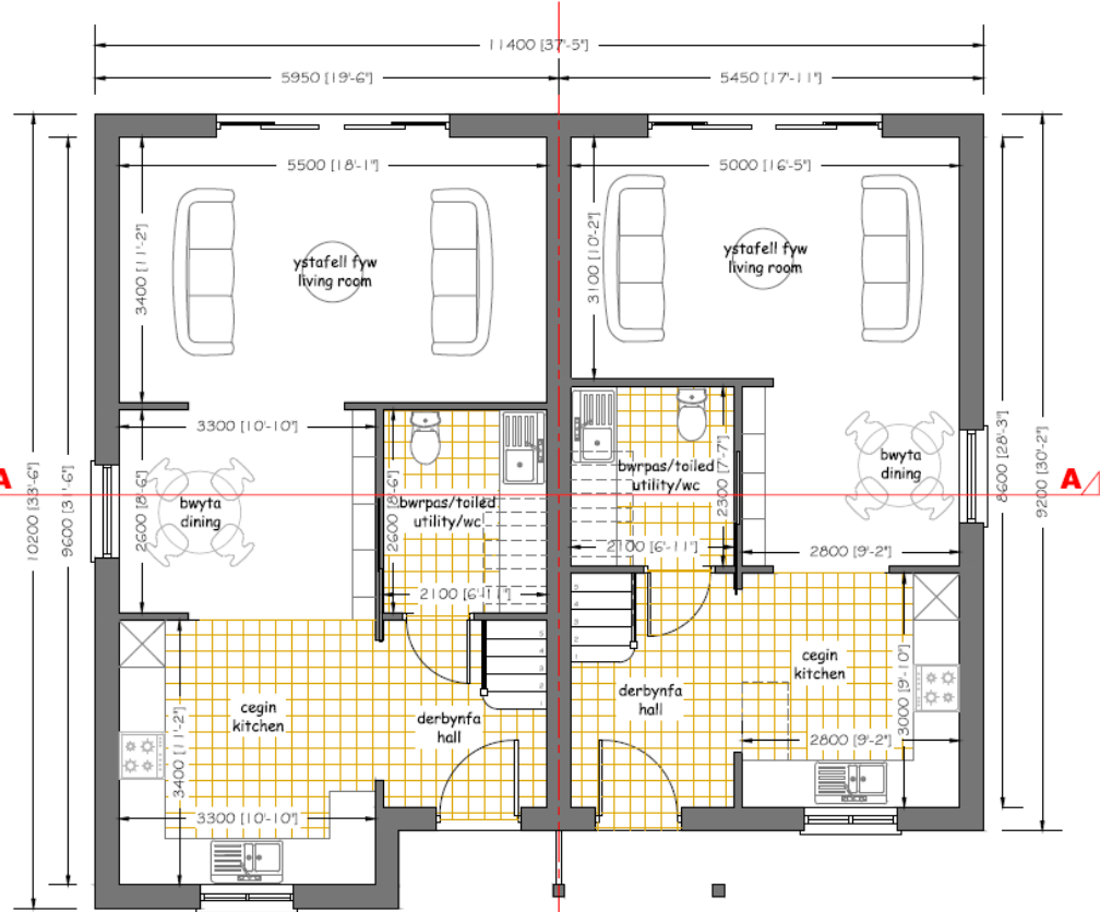
■ llawr waed ground floor - 1:50 Total Floor Area of No 1 & 3: 117 m 2 / 1,259 ft 2 Total Floor Area of No 2 & 4: 100 m 2 / 1,076 ft 2
